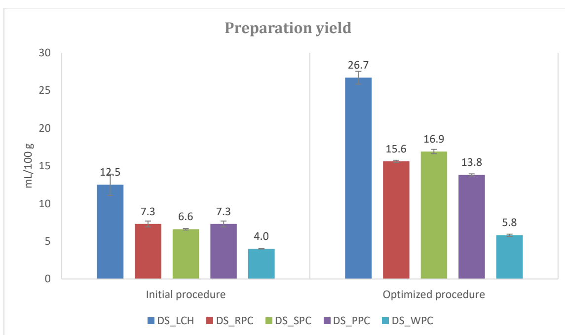
Figure 3. Preparation yields for the dietary supplements obtained by initial procedure vs optimised procedure
